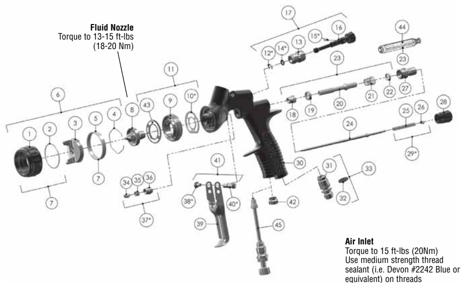
CHART 1 Air Cap Replacement Parts
