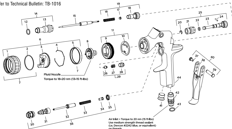
CHART 1: Fluid Nozzle & Fluid Needle Replacement Parts
