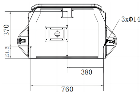
Fig. 5-3 Fixing dimension diagram
