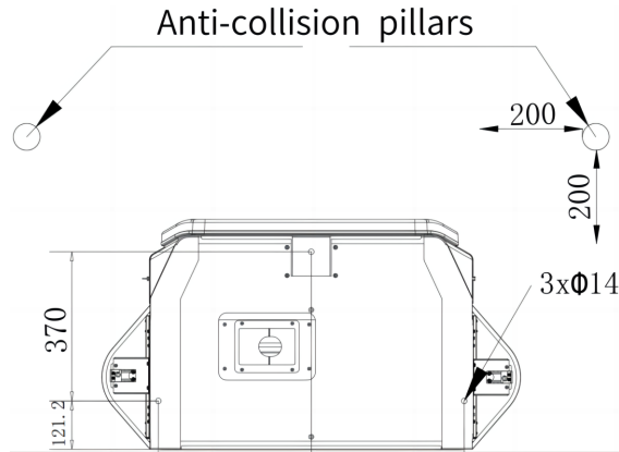
Fig. 5-4 Anti-collision pillars
