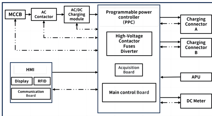
Fig. 4-2 Block diagram of BoostQ
