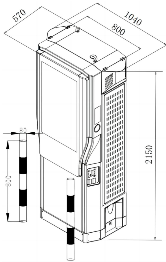
Fig. 5-1 Dimensions of BoostQ
