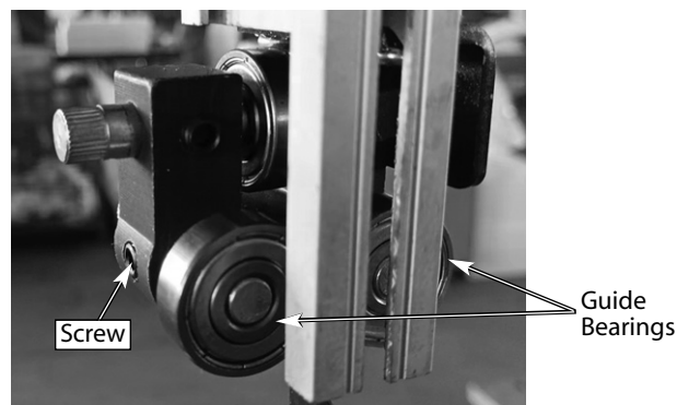
Figure 15 - Adjusting the guide bearings.
