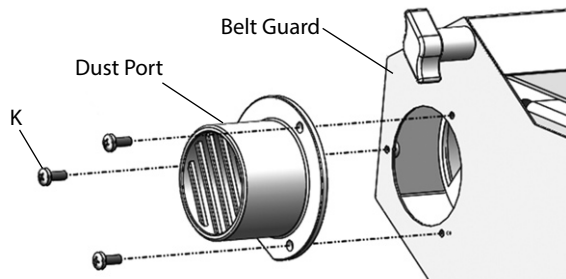
Figure 3 – Install sanding belt dust port.
