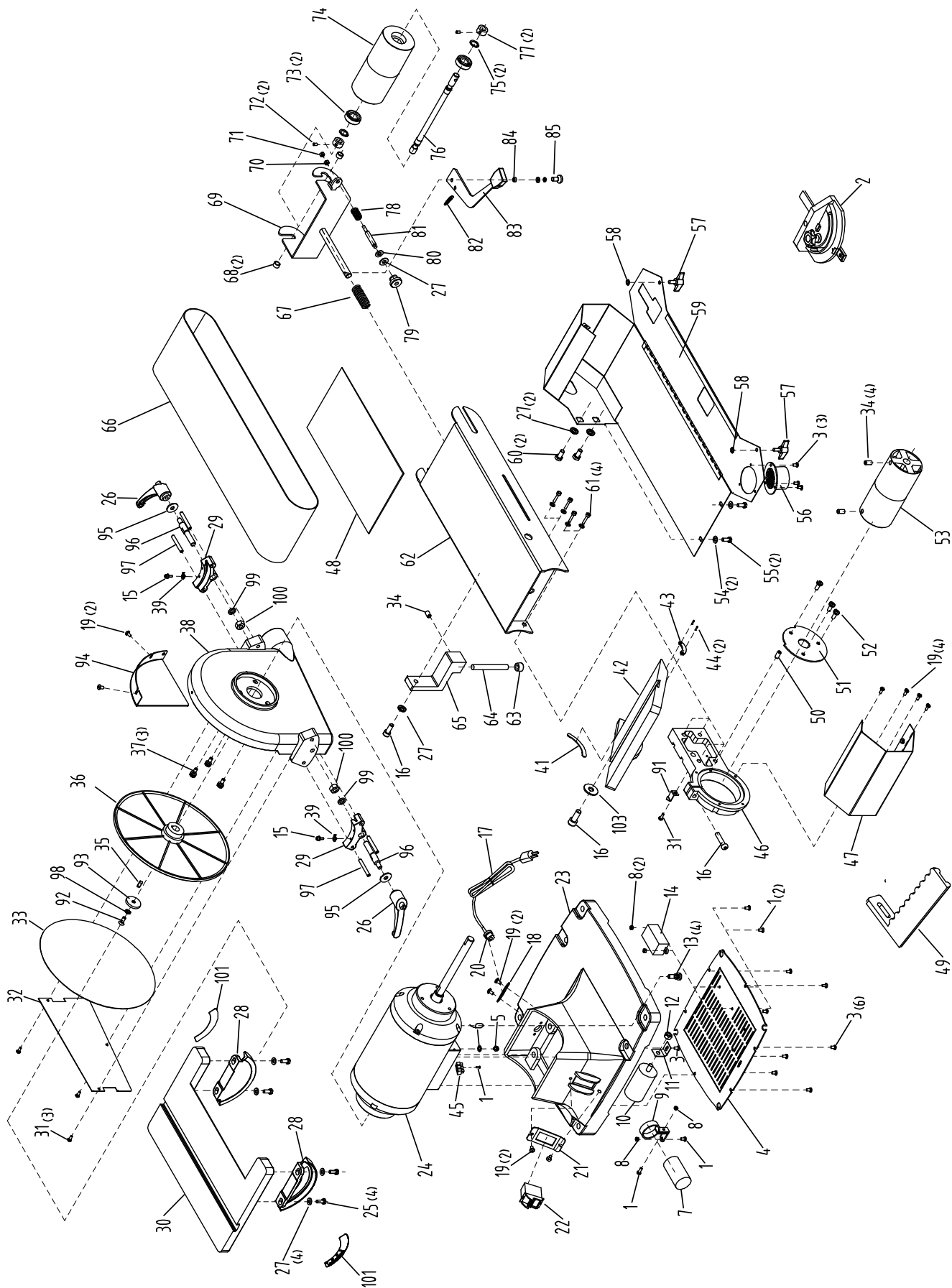
Figure 8 – Replacement parts illustration for belt/disc sander.
