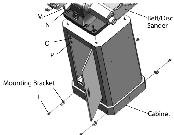
Figure 4 – Install machine to cabinet.
