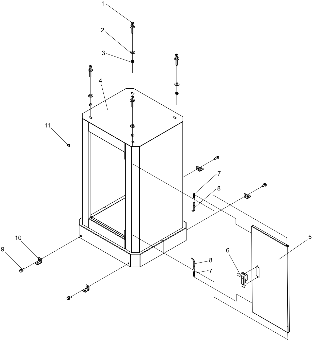
Figure 9 – Replacement parts illustration for cabinet.
