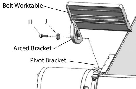
Figure 2 – Install sanding belt worktable.
