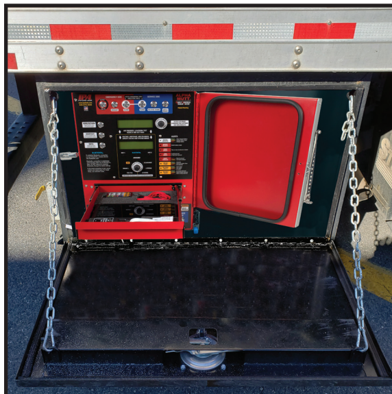
#5611A-RT8 Service-Truck Model Shown
